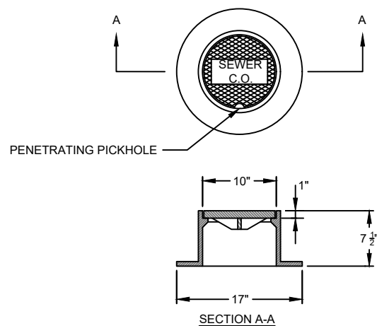
PROTECTIVE CASTING INSPECTION PORT
