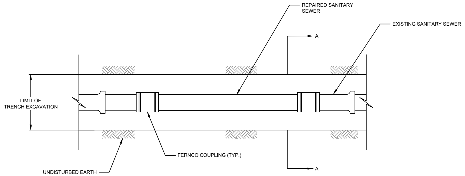
PLAN
